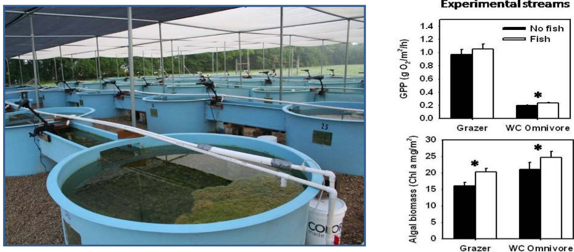
Fig. 10. Left: Konza experimental stream facility. There are 36 single separate recirculating pool-riffle units that mimic nearby natural stream pool sizes and riffle depths as well as hyporheic subsurface area A_s/A . Right: Contrasted effects of grazers and water-column minnows on gross primary productivity (GPP) and algal biomass across multiple experiments in this facility (asterisks indicate significant effects of consumers). In general, fishes stimulated biomass and GPP in experimental streams, which we hypothesize is due to increased nutrient recycling in the presence of consumers. From Bertrand 2007.
